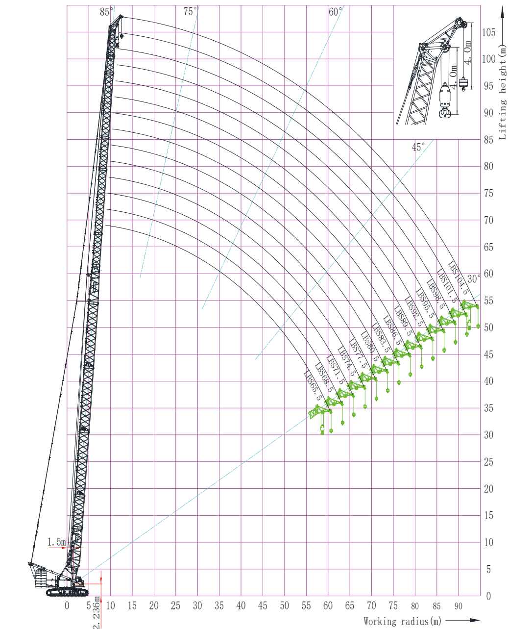
Light boom working condition_light boom single top aux. hook working range (with light boom main hook, LBS/2)
