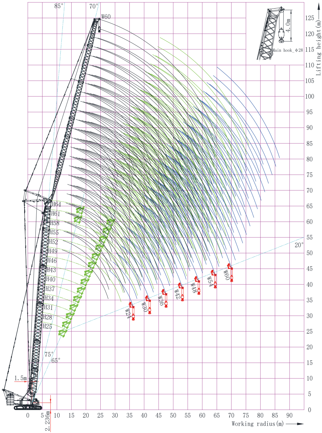
Tower jib working condition_ tower jib main hook working range (without boom pulley block and tower jib single top, HW/1)
